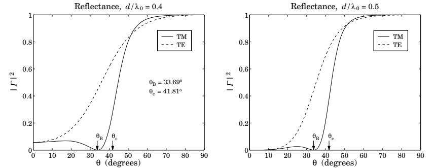
Fig. 8.4.4 Reflectance versus angle of incidence.
